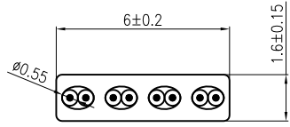
SECTION: A-A SCALE 4:1
